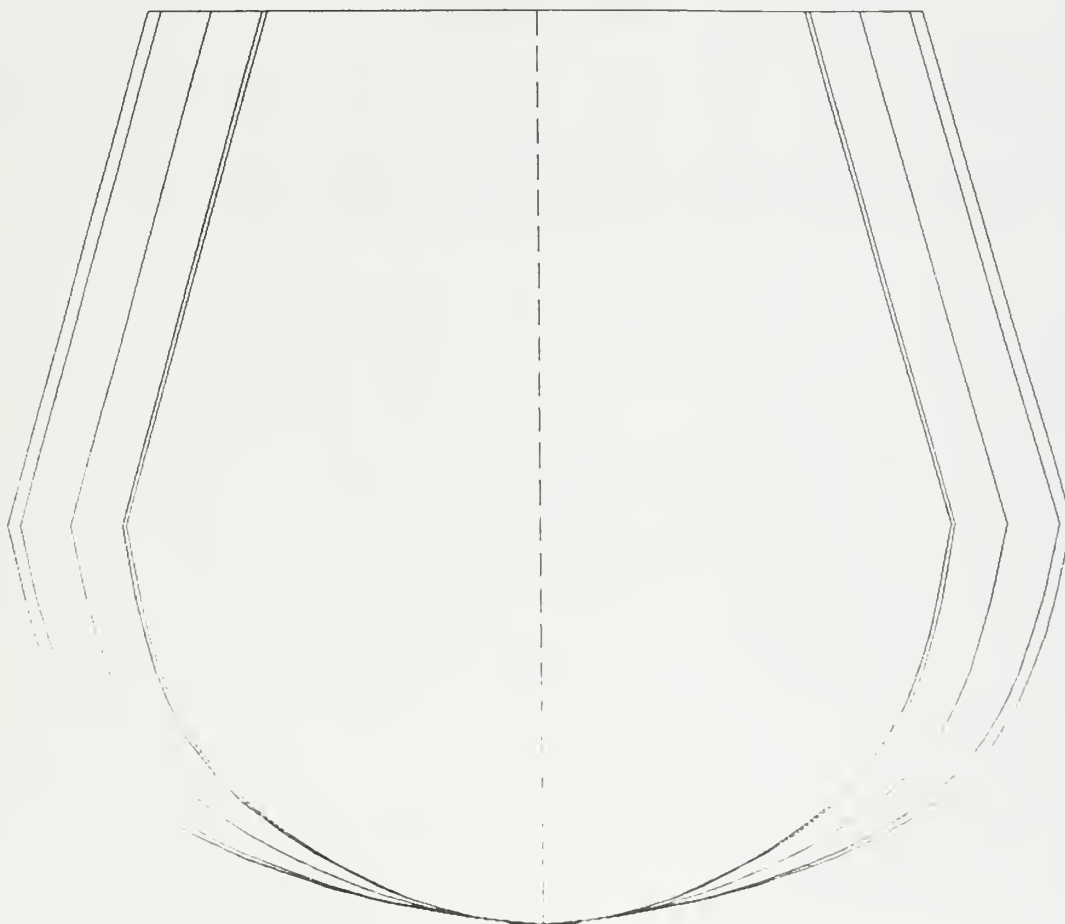
COMP_C.C Body Plan (1 component) Scale = 1:100
